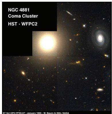
NGC4881
